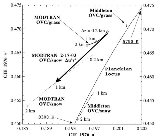
Fig. 18. MODTRAN simulations of stratus overcast u', v' chromaticities at the zenith as functions of cloud \Delta z and the underlying surface's spectral reflectance r_\lambda . The thick arrow indicates MODTRAN's prediction of the chromaticity shift caused by changing the surface from grass to snow for Fig. 19's observed changes in cloud \Delta z . For historical purposes, we also include overcast chromaticities simulated by Middleton. 4
