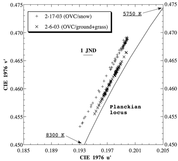
Fig. 19. Scatterplot of overcast u', v' chromaticities calculated from zenith L_\lambda at Owings during stratus overcasts on 2-6-03 and 2-17-03; h_0 ranges from 14.4^\circ – 20.5^\circ . Only on 2-17-03 was the ground snow-covered. Compare these measured chromaticities with MODTRAN simulations in Fig. 18.
