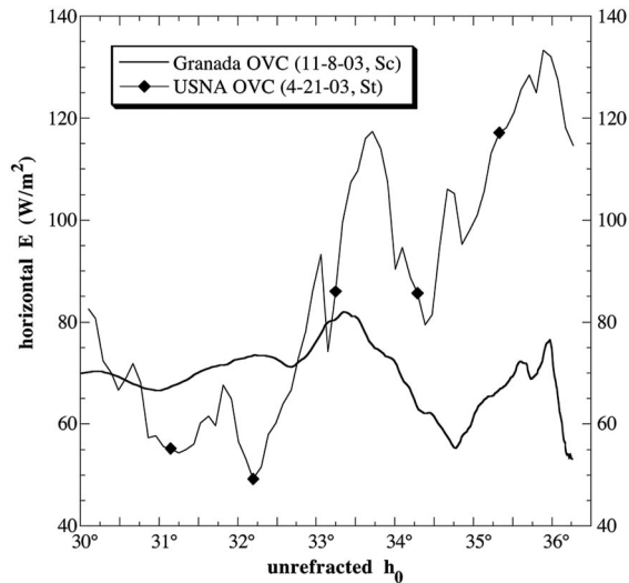
Fig. 2. Spectrally integrated horizontal irradiances E versus h_0 for Fig. 1's two overcasts. Integrals are calculated from 380–780 nm in 4 nm steps.
