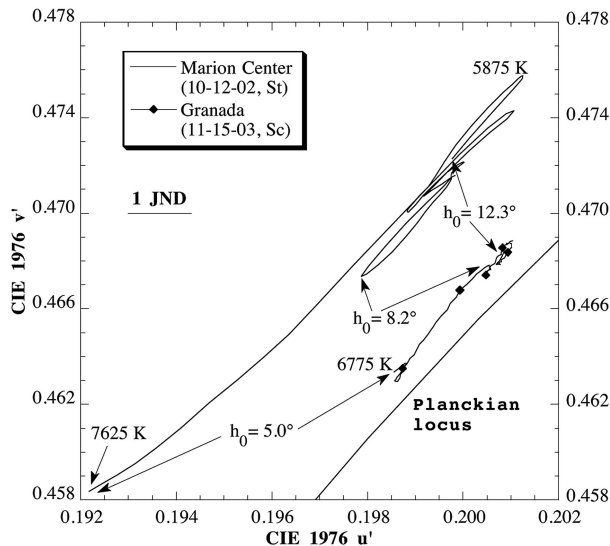
Fig. 17. Temporal trends in overcast u', v' chromaticities calculated from E_\lambda near Marion Center, Pennsylvania, on 10-12-02 and at Granada on 11-15-03; h_0 ranges from 5.0^\circ – 12.3^\circ .
