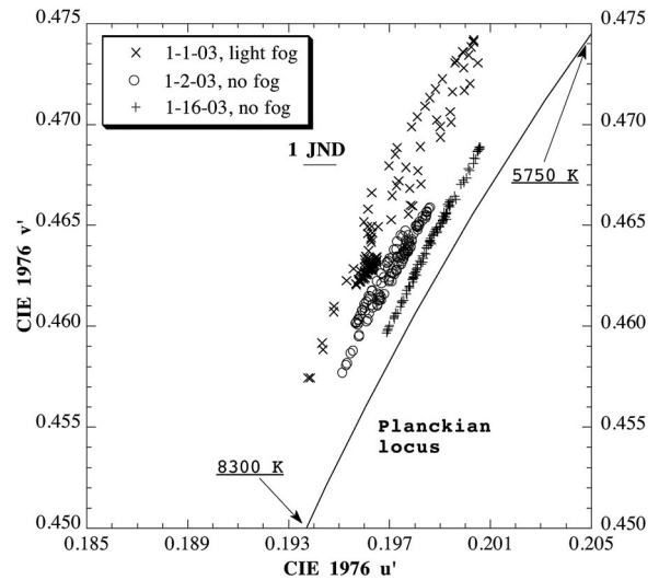
Fig. 20. Scatterplot of overcast u', v' chromaticities calculated from zenith L_\lambda at Owings during stratus overcasts on 1-1-03, 1-2-03, and 1-16-03. The ground was snow-free on all days; h_0 ranges from 12.3^\circ – 20.2^\circ .
