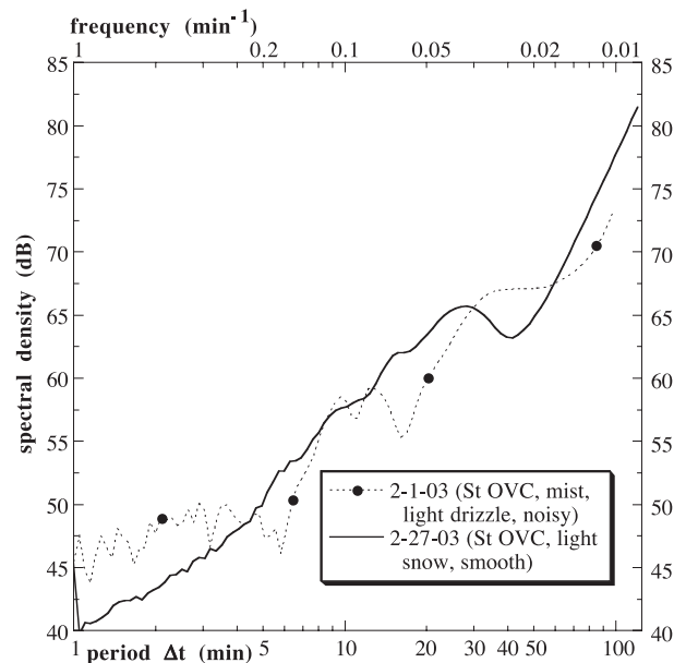
Fig. 8. Power spectra (SDF) of stratus overcast L_v as functions of period \Delta t or temporal frequency 1/\Delta t at Owings on 2-1-03 and 2-27-03 (see Fig. 7 for corresponding L_v time series).
