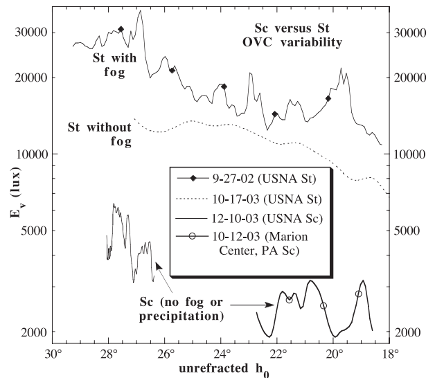
Fig. 11. Horizontal illuminance E_v as a function of h_0 for several stratus and stratocumulus overcasts at USNA (9-27-02, 10-17-03, and 12-10-03) and at a rural site near Marion Center, Pennsylvania (10-12-03).
